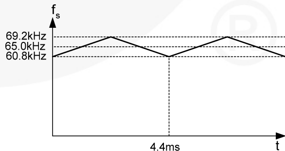
Figure 27. Frequency Hopping
