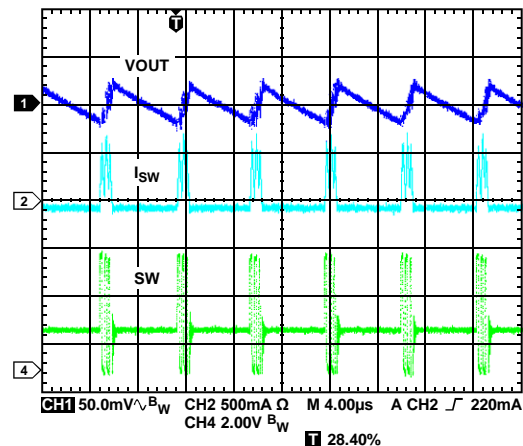
Figure 20. Typical Waveforms, V_{OUT2} = 1.8V , I_{OUT2} = 30mA , Auto Mode
