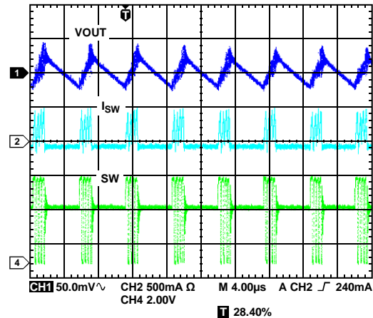
Figure 19. Typical Waveforms, V_{OUT1} = 3.3V , I_{OUT1} = 30mA , Auto Mode
