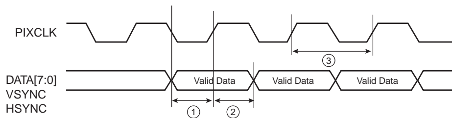
Figure 54-62. ISI Timing Diagram
