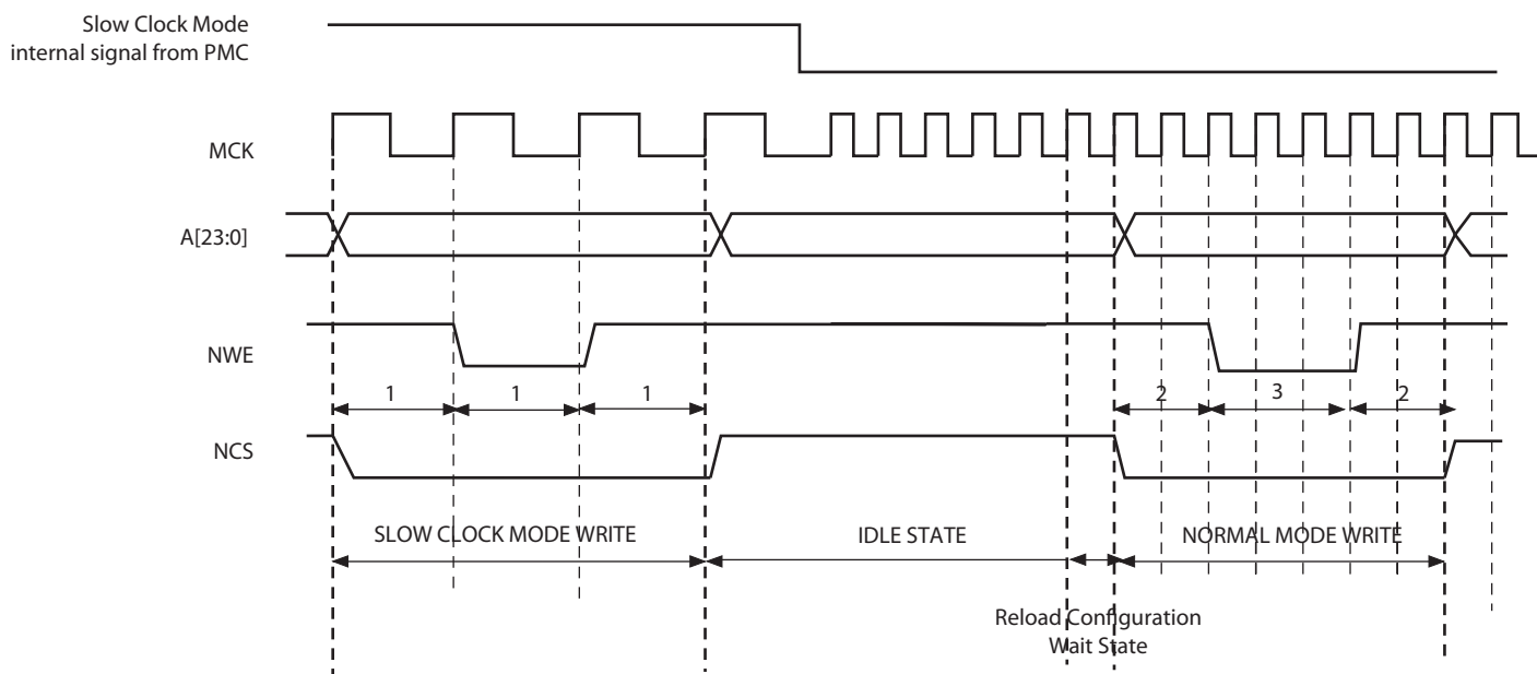
Figure 34-32. Recommended Procedure to Switch from Slow Clock Mode to Normal Mode or from Normal Mode to Slow Clock Mode
