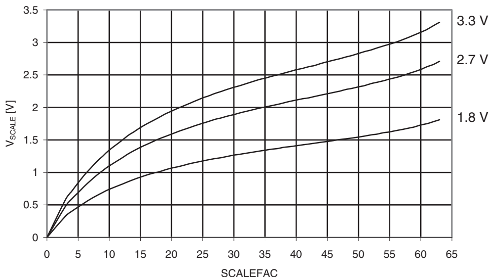
Figure 34-4. Analog Comparator Voltage Scaler vs. Scalefac T = 25°C
