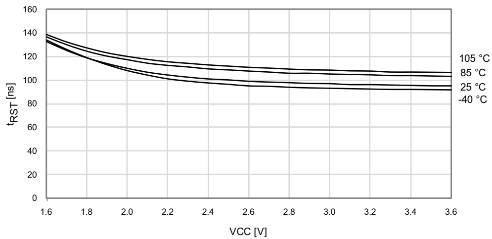
Figure 34-190. Minimum Reset Pin Pulse Width vs. V CC
