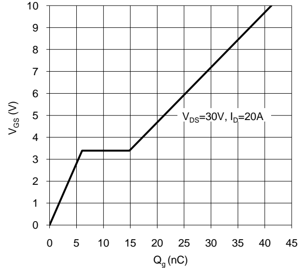
Figure 10. Gate Charge
