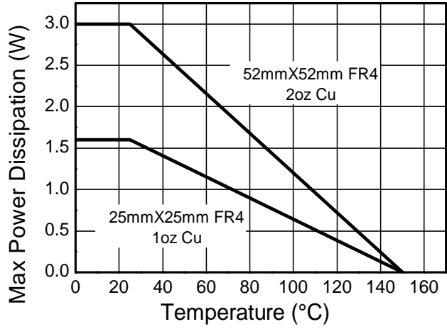
Derating Curve
