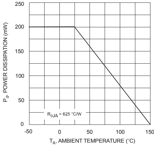
Fig. 1 Derating Curve
