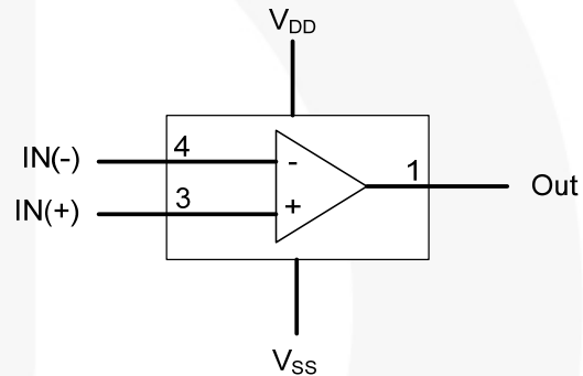
Figure 1. Functional Diagram
