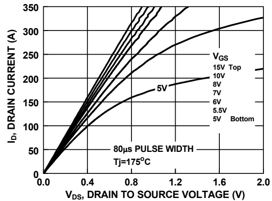
Figure 10. Saturation Characteristics
