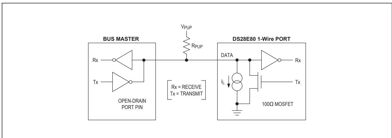
Figure 7. Hardware Configuration
