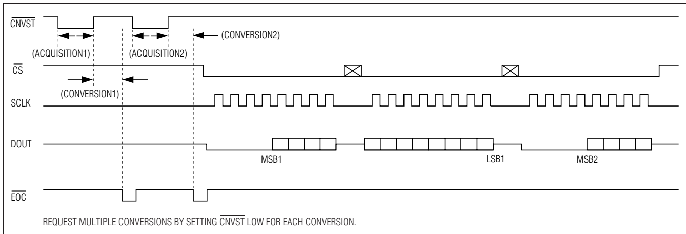
Figure 5. Clock Mode 01
