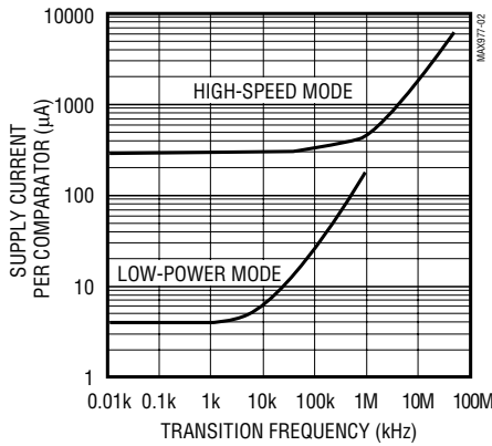
SUPPLY CURRENT PER COMPARETOR vs. OUTPUT TRANSITION FREQUENCY
