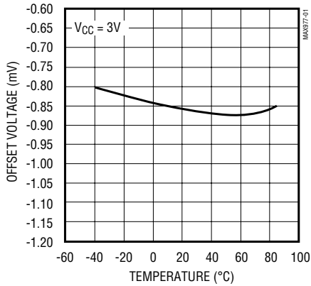
LOW-POWER OFFSET VOLTAGE vs. TEMPERATURE
