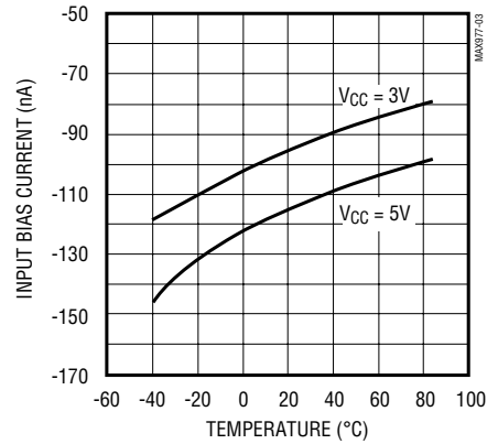
HIGH-SPEED INPUT BIAS CURRENT vs. TEMPERATURE
