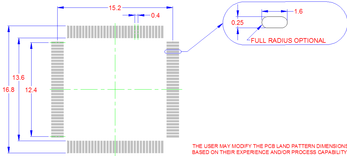
Figure 16.2 128-VTQFP Recommended PCB Land Pattern
