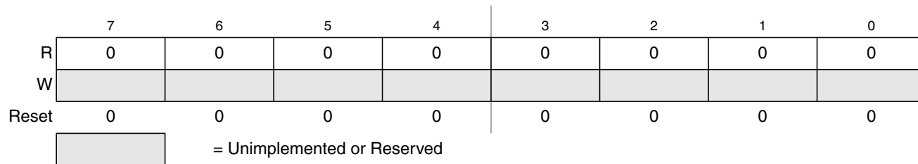
Figure 31-23. Flash Reserved5 Register (FRSV5)
