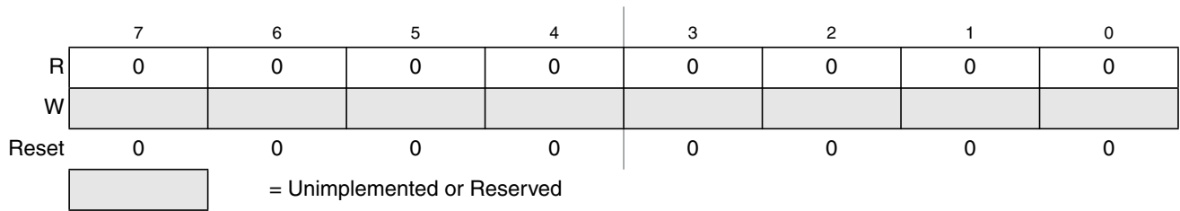
Figure 29-20. Flash Reserved3 Register (FRSV3)
