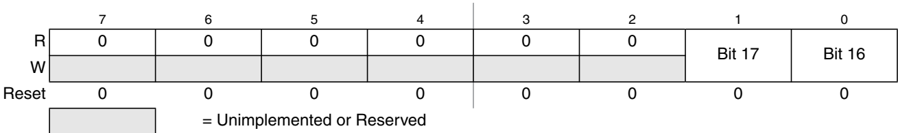
Figure 8-16. Debug Comparator Address High Register (DBGXAH)
