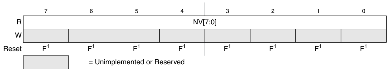
Figure 31-22. Flash Option Register (FOPT)
