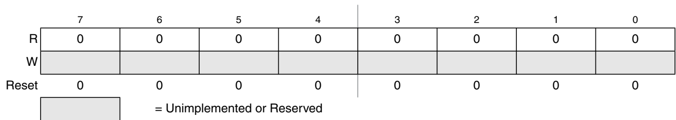
Figure 31-21. Flash Reserved4 Register (FRSV4)
