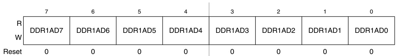
Figure 2-54. Port AD Data Direction Register (DDR1AD)
