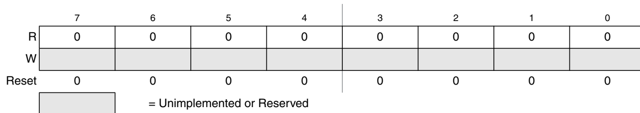
Figure 31-24. Flash Reserved6 Register (FRSV6)
