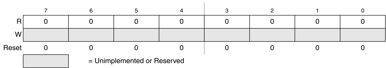
Figure 31-20. Flash Reserved3 Register (FRSV3)
