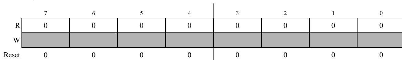
Figure 2-21. PIM Reserved Register
