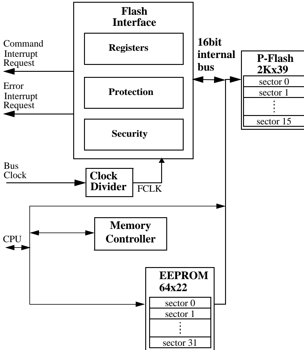
Figure 20-1. FTMRZ8K128 Block Diagram
