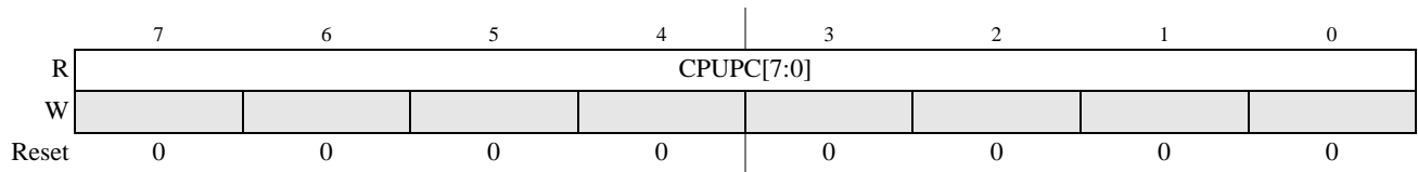
Figure 3-7. Captured S12ZCPU Program Counter (MMCPCH, MMCPCL, MMCPCL)
