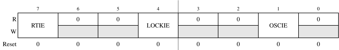
Figure 8-9. S12CPMU_UHV_V5 Interrupt Enable Register (CPMUINT)
