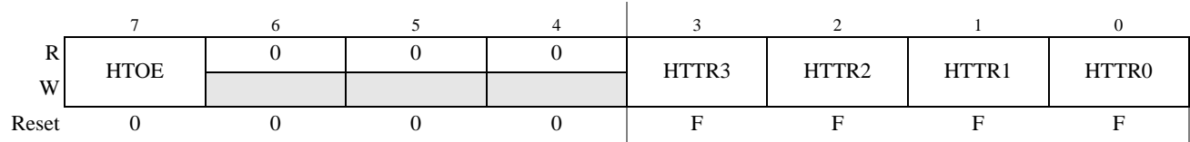
Figure 8-26. High Temperature Trimming Register (CPMUHTTR)
