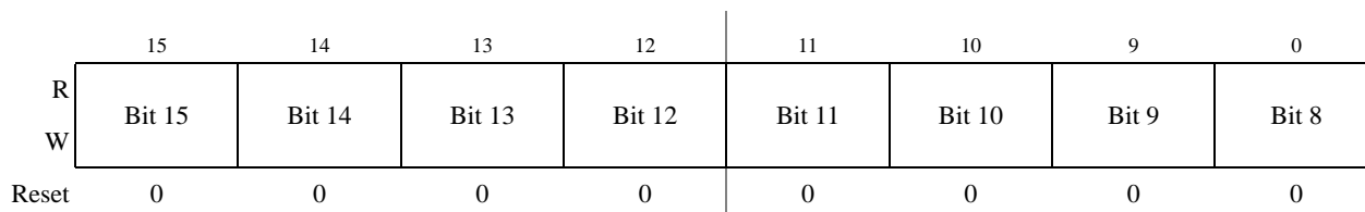
Figure 11-18. Timer Input Capture/Output Compare Register x High (TCxH)
