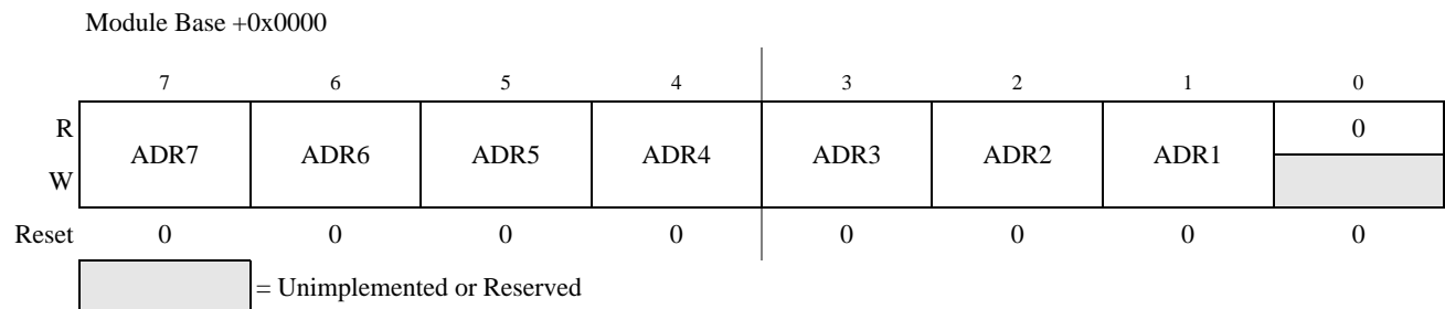
Figure 16-3. IIC Bus Address Register (IBAD)
