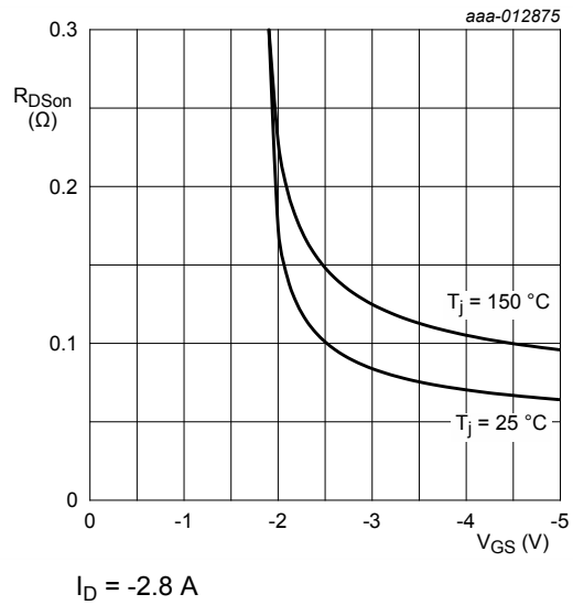
Fig. 9. Drain-source on-state resistance as a function of gate-source voltage; typical values I_D = -2.8\text{ A}
