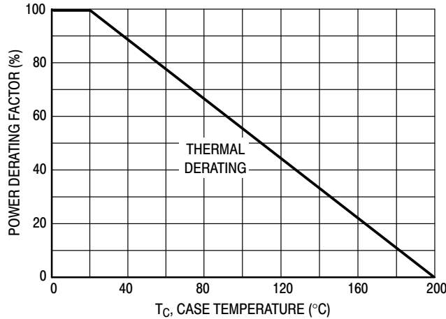
Figure 10. Power Derating
