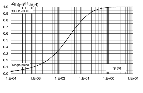
Figure 8: Relative variation of thermal impedance junction to lead versus pulse duration (SOD123Flat)
