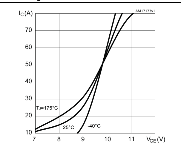
Figure 9. Transfer characteristics
