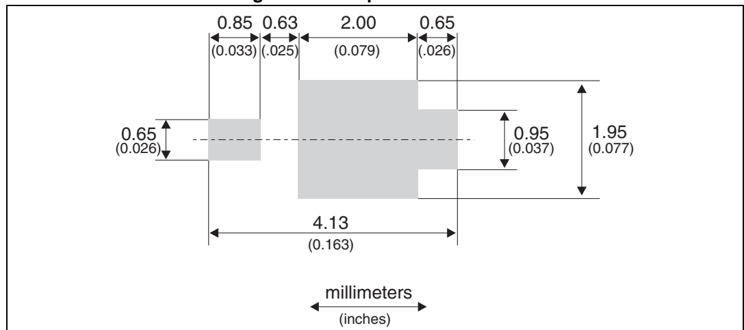
Figure 21. Footprint dimensions
