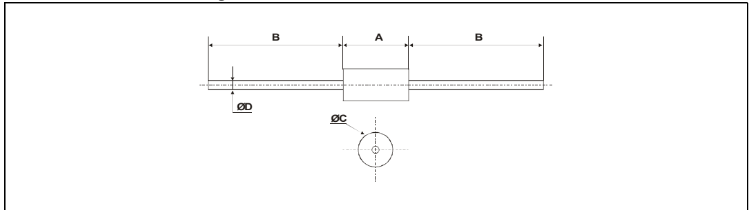
Figure 27. DO-201 dimension definitions
