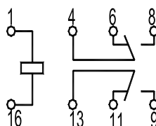
Wiring diagram (Bottom views)
